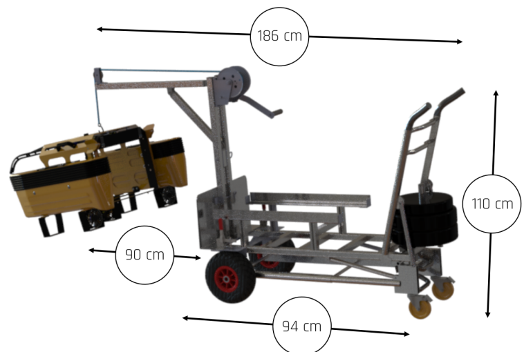
Figure b : Trolley unfolded setup
