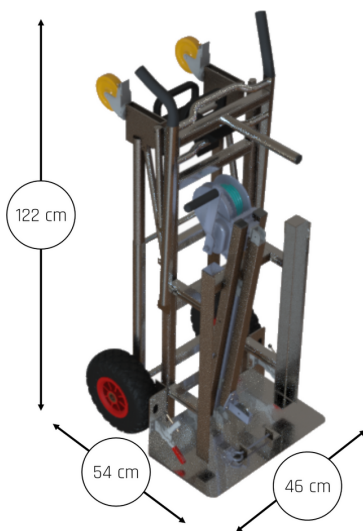
Figure a : Trolley folded setup
